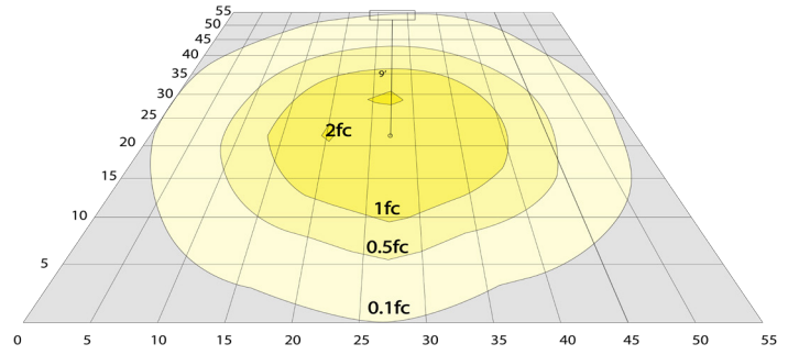
36W, 5000K Area 55'x 55' Mounting Height: 9'
